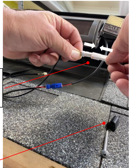
Snap Cables Together
